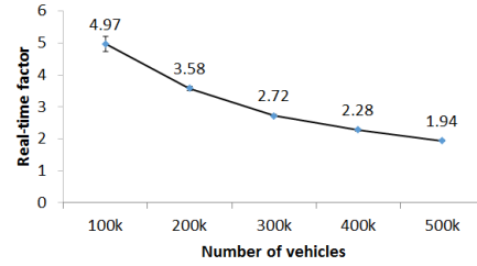
Fig. 15. Real-time factor with the number of vehicles. There are 30 workers. The look-ahead distance is set to 100 metres. The step length is 0.2 second. Simulations run with decentralized synchronization.
